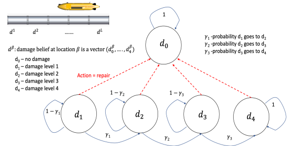
Figure 5. Markov chain for the damage level of each location of the pipeline.
