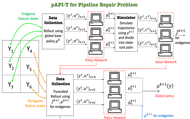
Figure 7. Algorithm for applying pAPI-T to our pipeline repair problem.
